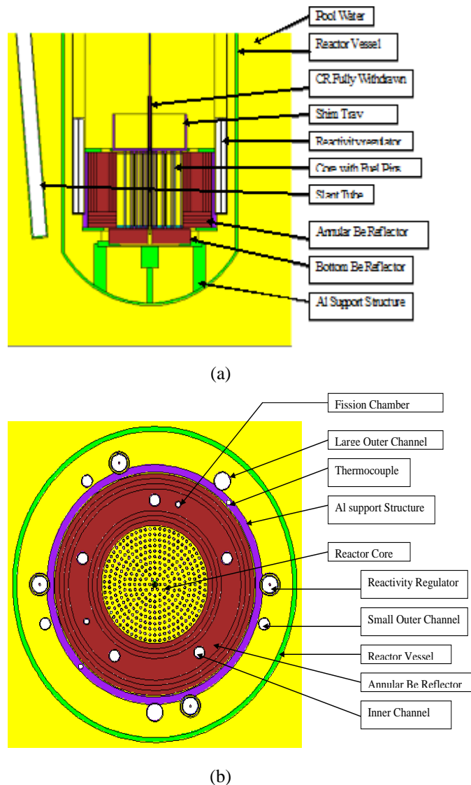
Fig. 1 MCNP Axial and Radial view of NIRR-1
