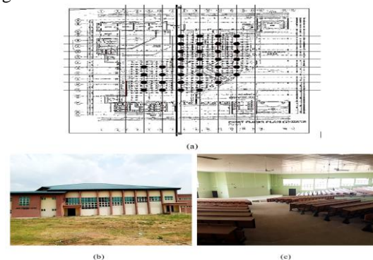
Fig. 3. UAM lecture theatre (969 capacity): (a) Floor plan; (b) Exterior view; (c) Interior view.
